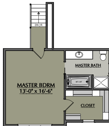
2ND FLOOR
