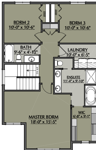
2ND FLOOR 914.5 SQ. FT.
